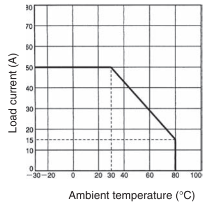
G3PA-450B-VD-2
